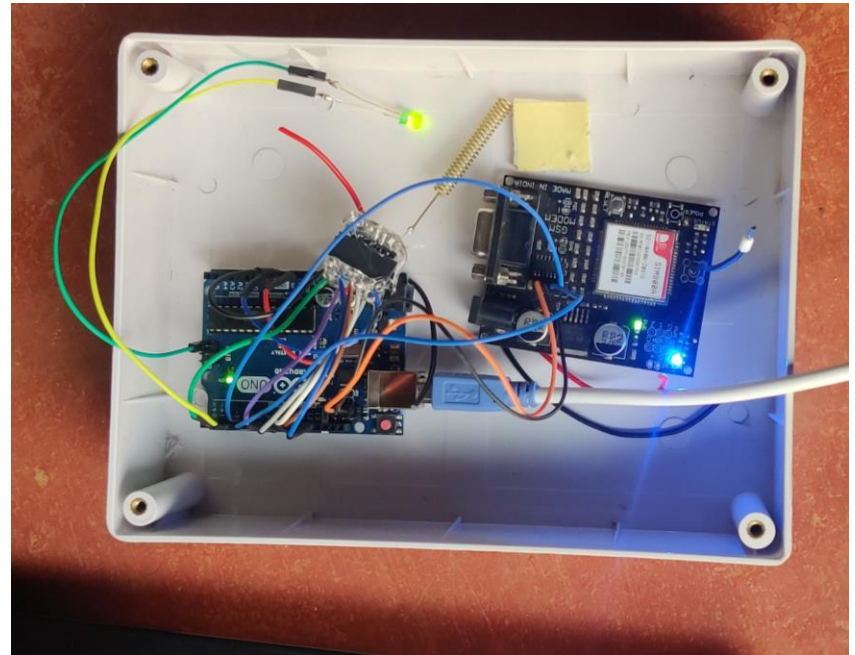
Base station
